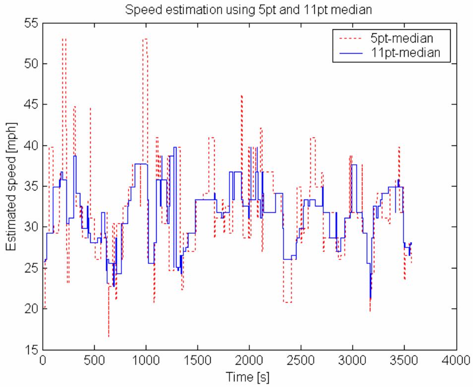
Figure 4 Vehicle speed using 5-point and 11-point median
